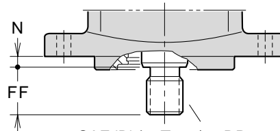
SAE 'B' (13T, 16/32 DP; class 1, flat root, side fit) Spline shaft S (SAE J498b)
