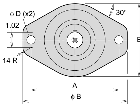
Mounting flange S SAE 'B' (SAE J744c)
