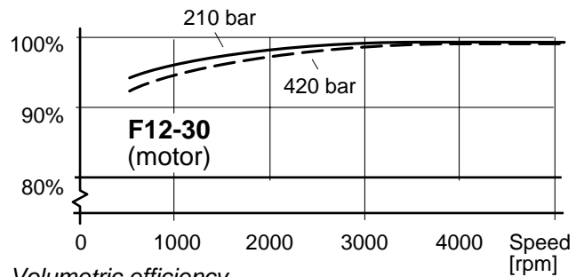
Volumetric efficiency.
