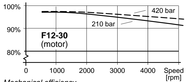
Mechanical efficiency.
